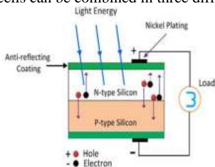
Fig 1 photovoltaic cell
